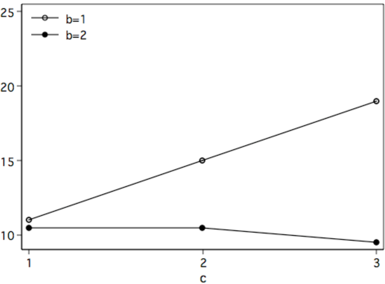
b \cdot c at a=1
